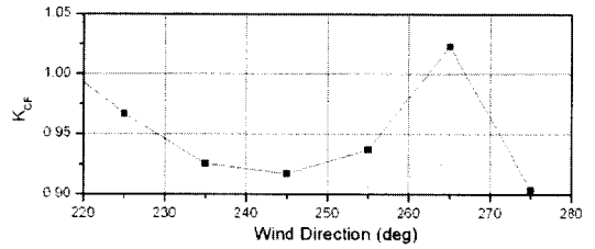
Fig. 9 Flow correction factor by bin-averaging ratio method
