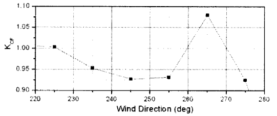
Fig. 10 Flow correction factor by least square method
