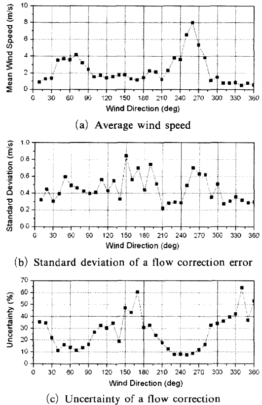
Fig. 14 Uncertainty allocation for a flow correction
