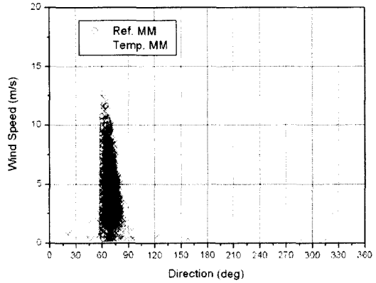
(a) East wind (60°~70°, sector #7)
