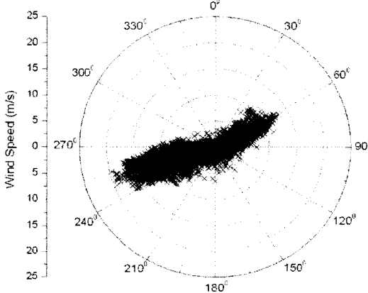
(b) Wind rose for the temporal meteorological mast
