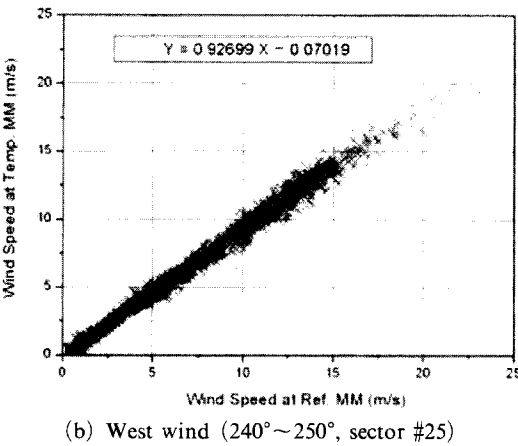
Fig. 8 The correlation of the wind data measured at two meteorological masts
