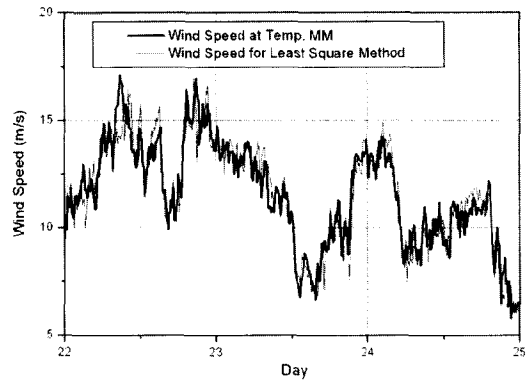
(b) Least square method
